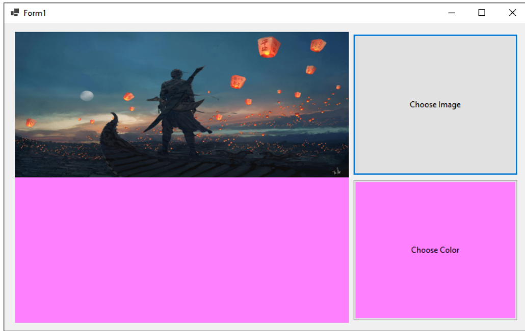
Figure 24: ImageButton logic
