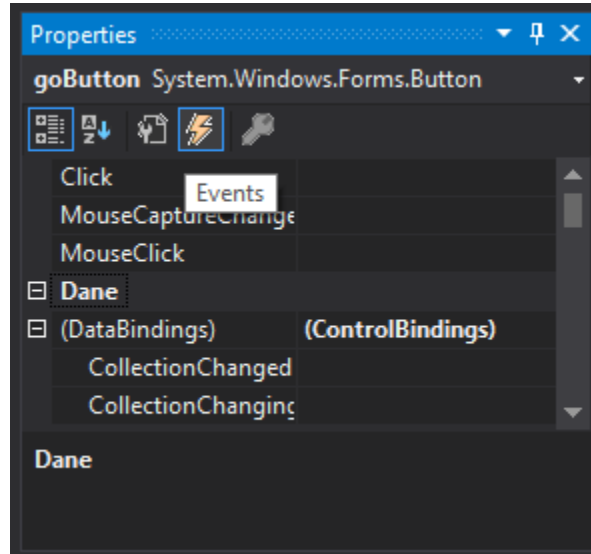
Figure 8: Button events
