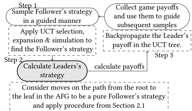
Figure 1: An outline of the O2UCT method.
