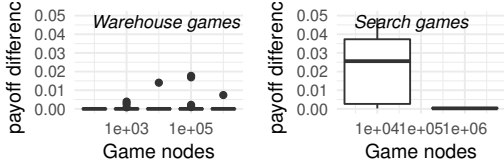
Figure 2: A difference in Leader’s payoffs between the SSE strategy and the O2UCT strategy w.r.t. the number of nodes.
