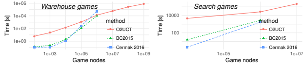
Figure 3: Computation times comparison.
